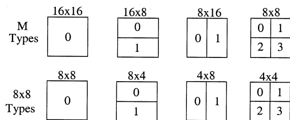
Fig. 12. Segmentations of the macroblock for motion compensation. Top: segmentation of macroblocks, bottom: segmentation of 8×8 partitions.
